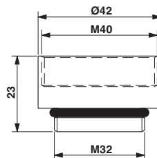
Dimensioned drawing
