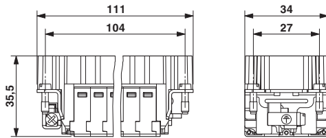
HC-B 24-ESTZ male insert
