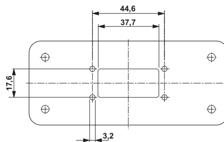
Panel cutout
