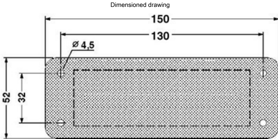
Adapter plate
