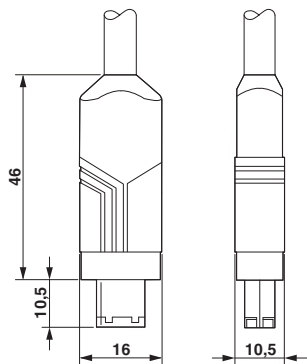
FireWire connector, standard
