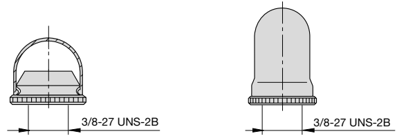
Reset button seal for 3/8", 27-thread, short X 201 285 01 (IP64) long X 200 799 01 (IP64)
