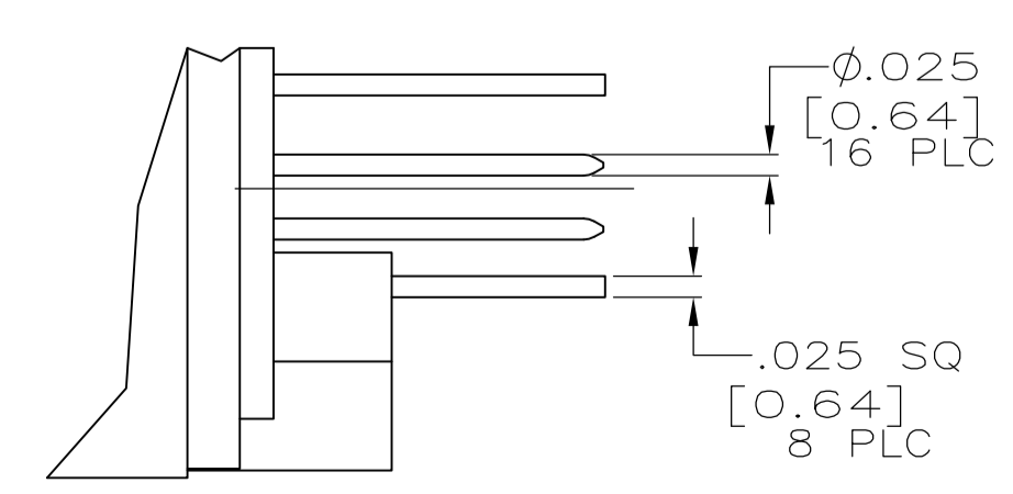
DETAIL T SCALE 4:1 SIZE 8 QUADRAX ONLY
