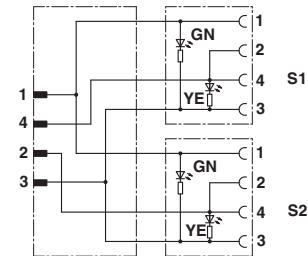
Contact assignment of the M12 plug and the M12 socket
