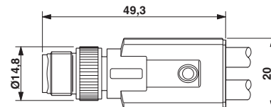
Dimensioned drawing
