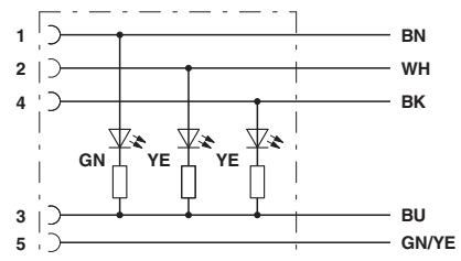
Circuit diagram
