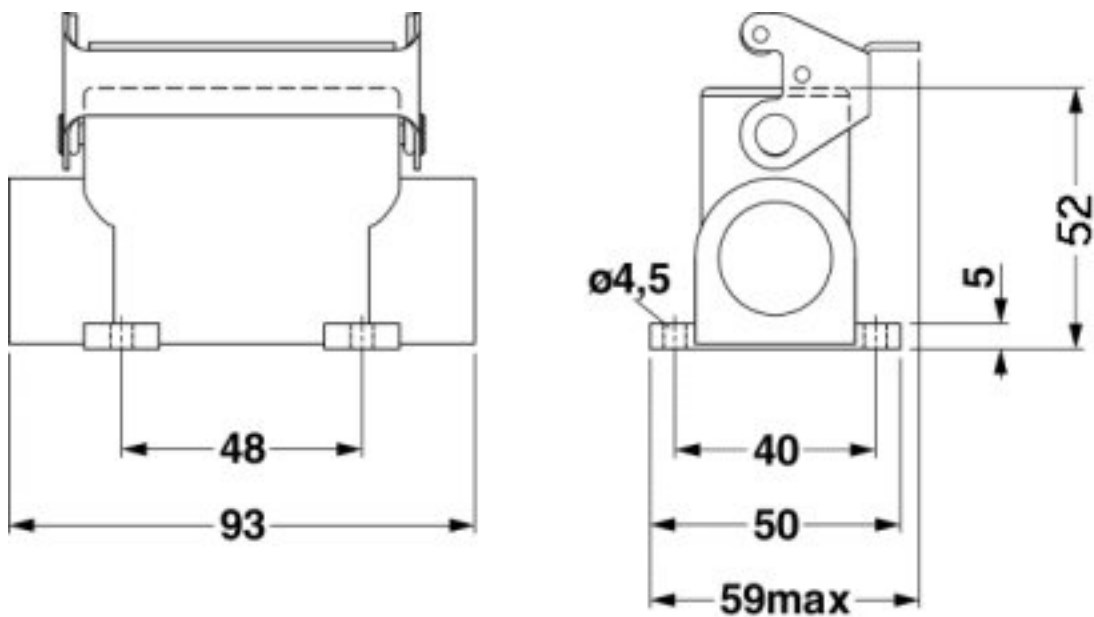
Dimensioned drawing
