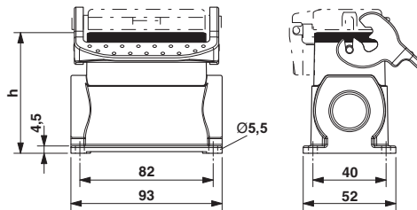
Dimensional drawing; h = 52 \text{ mm}
