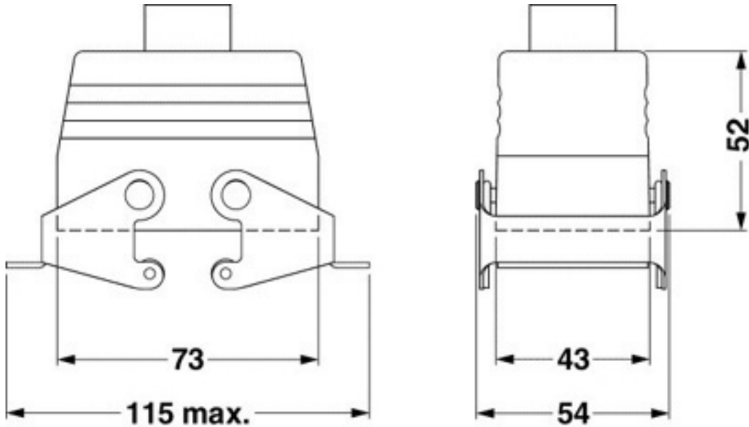
Dimensioned drawing
