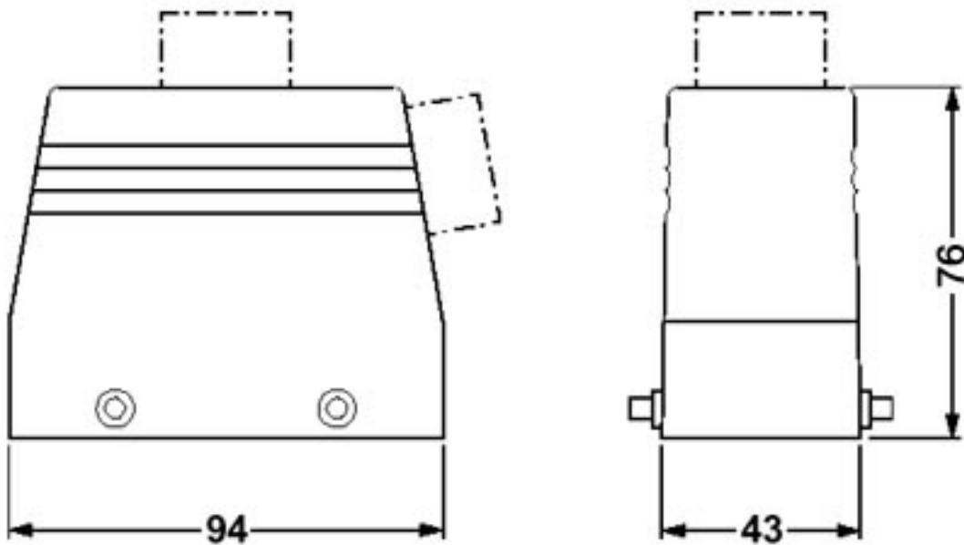
Dimensioned drawing
