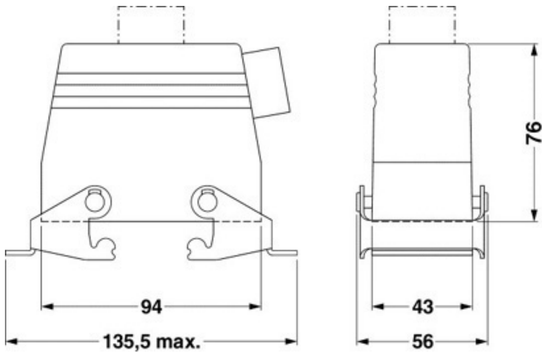
Dimensioned drawing
