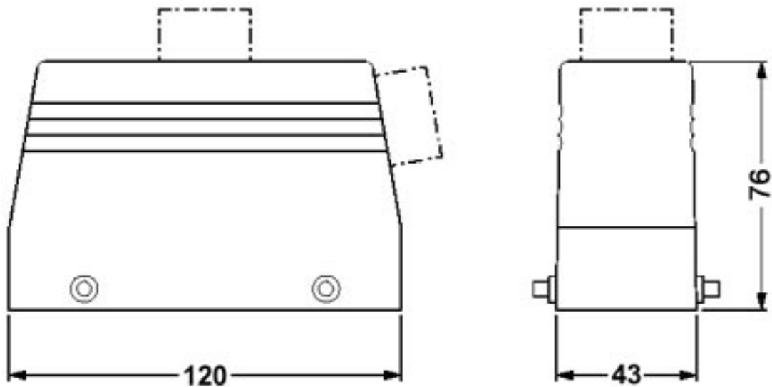
Dimensioned drawing
