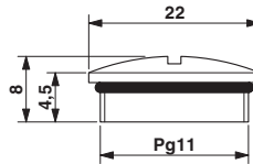
Filler plugs Pg11
