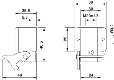
Dimensioned drawing
