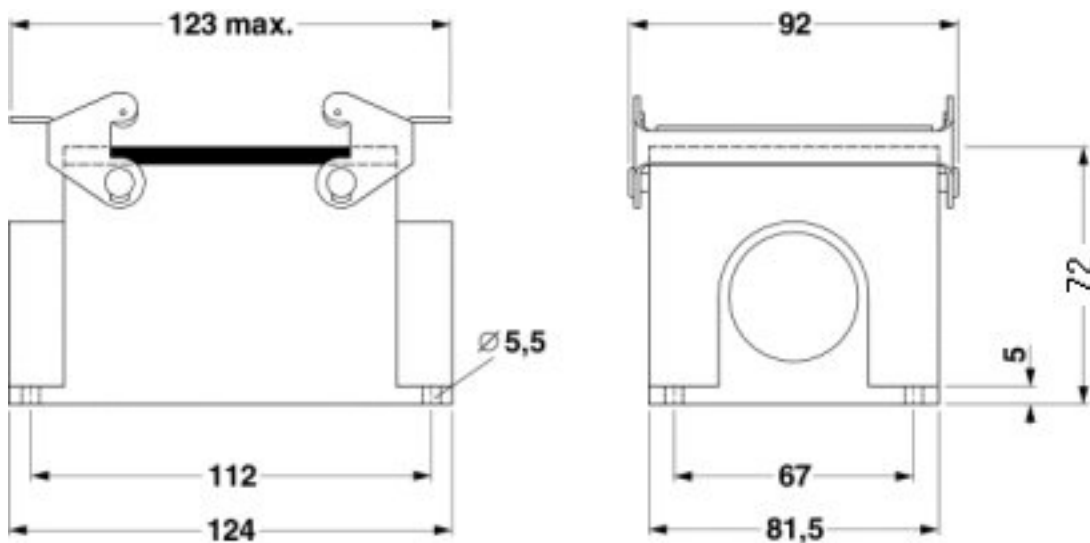
Dimensioned drawing
