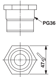
Dimensioned drawing
