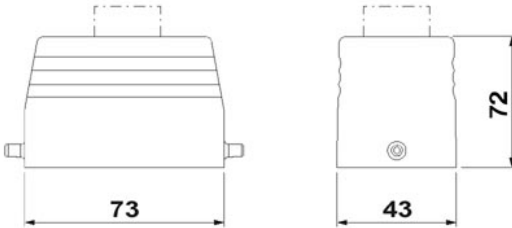
Dimensioned drawing
