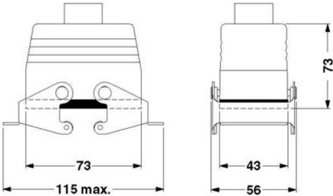
Dimensioned drawing
