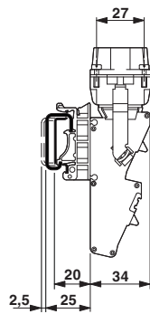
Dimensioned drawing
