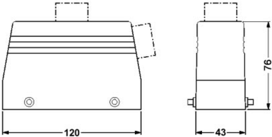
Dimensioned drawing
