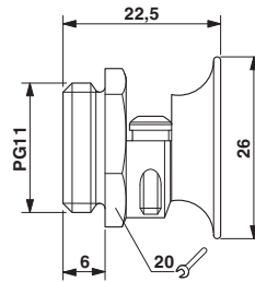
Dimensioned drawing
