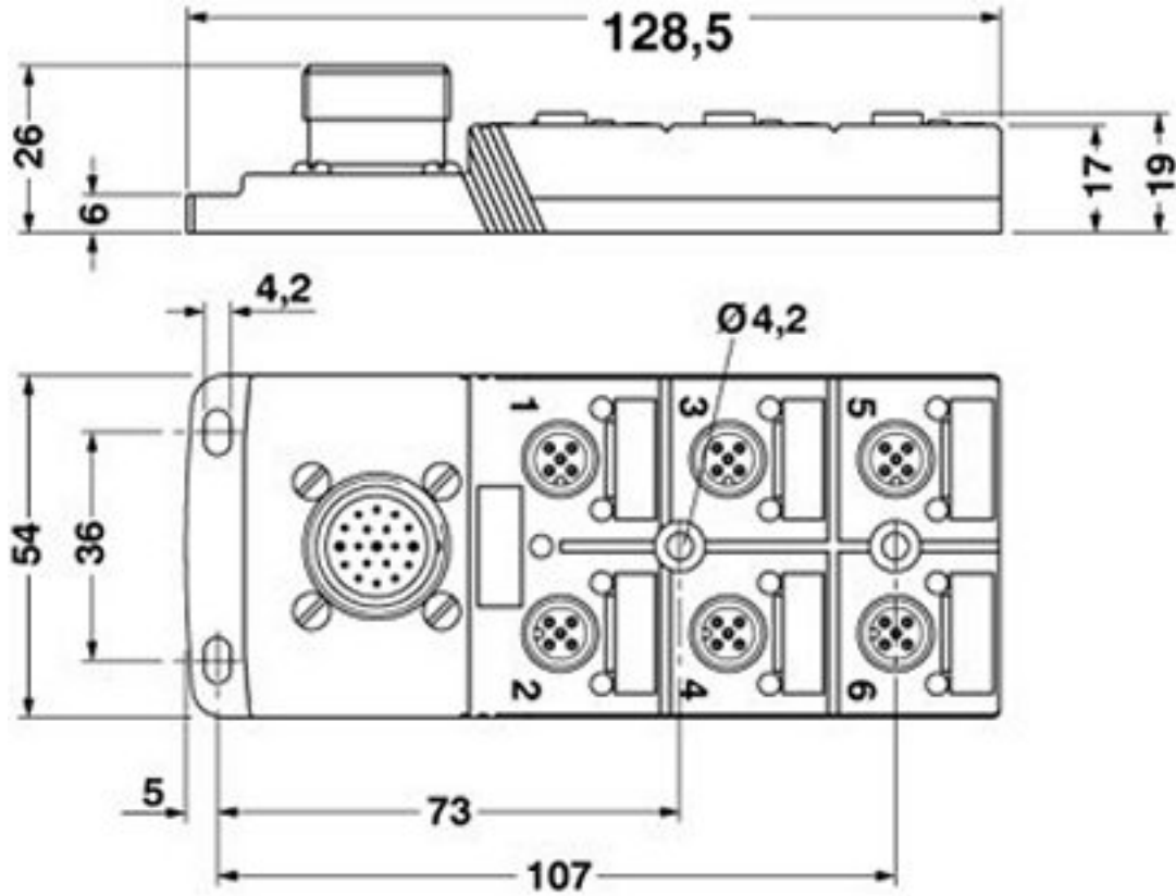
Dimensioned drawing
