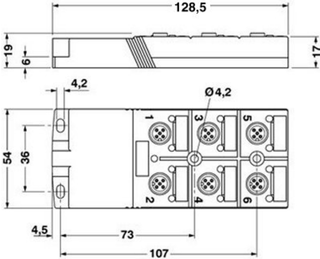
Dimensioned drawing
