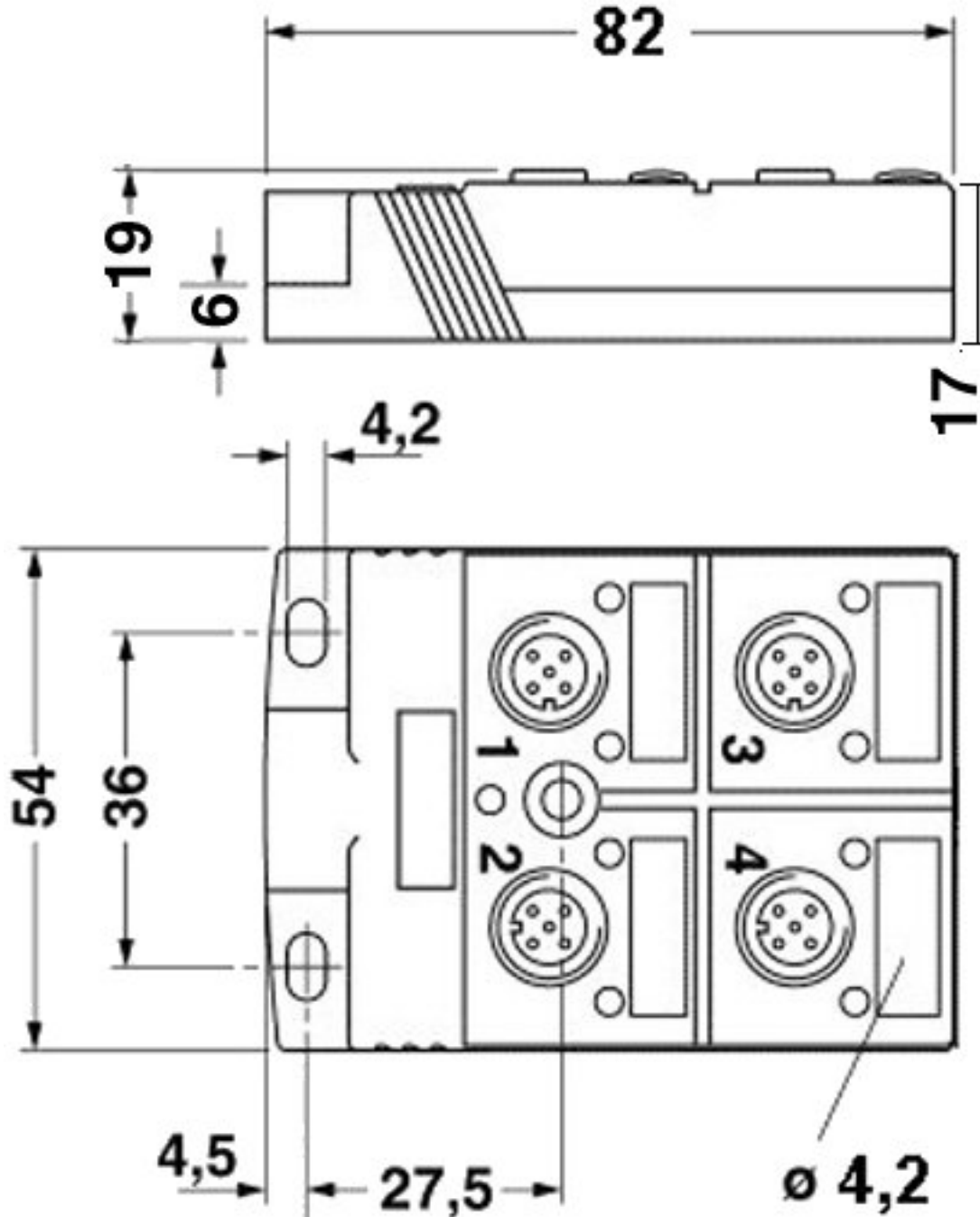
Dimensioned drawing
