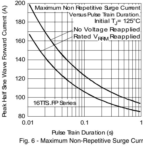
Fig. 6 - Maximum Non-Repetitive Surge Current
