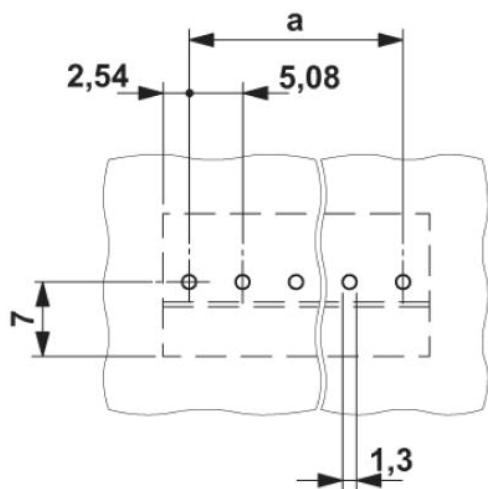
Drilling plan/solder pad geometry
