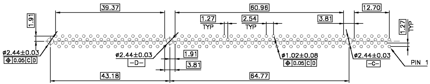
RECOMMENDED PCB LAYOUT (TOP VIEW) TOLERANCE: ±0.05, THICKNESS: 1.6mm
