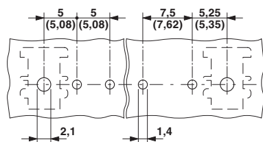
Drilling diagram
