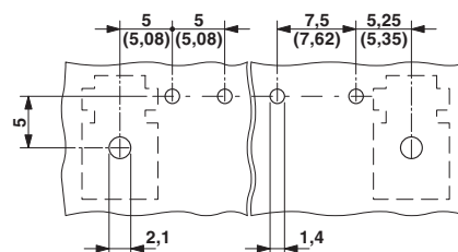
Drilling diagram
