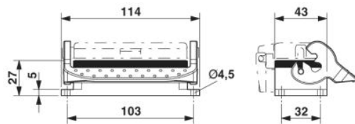
Dimensional drawing
