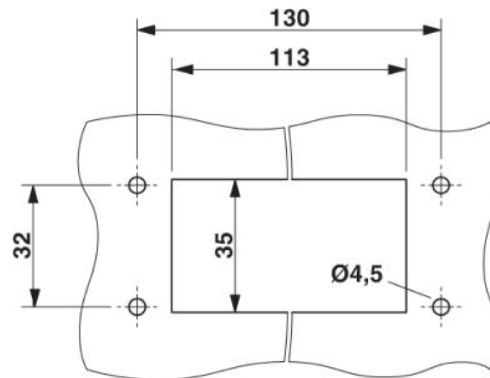
Panel cutout
