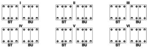
Coding for housings with two contact inserts
