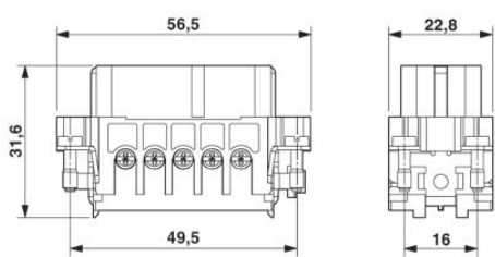
Female insert
