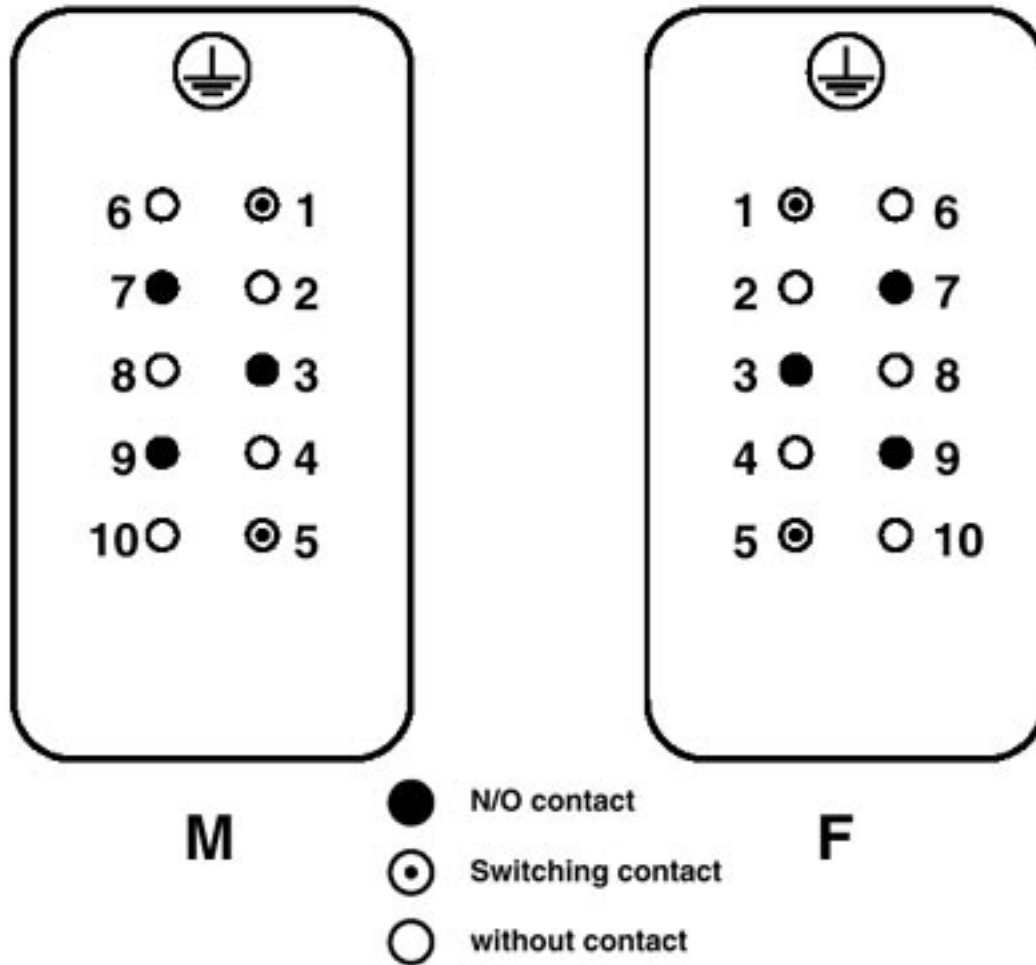
Schematic diagram
