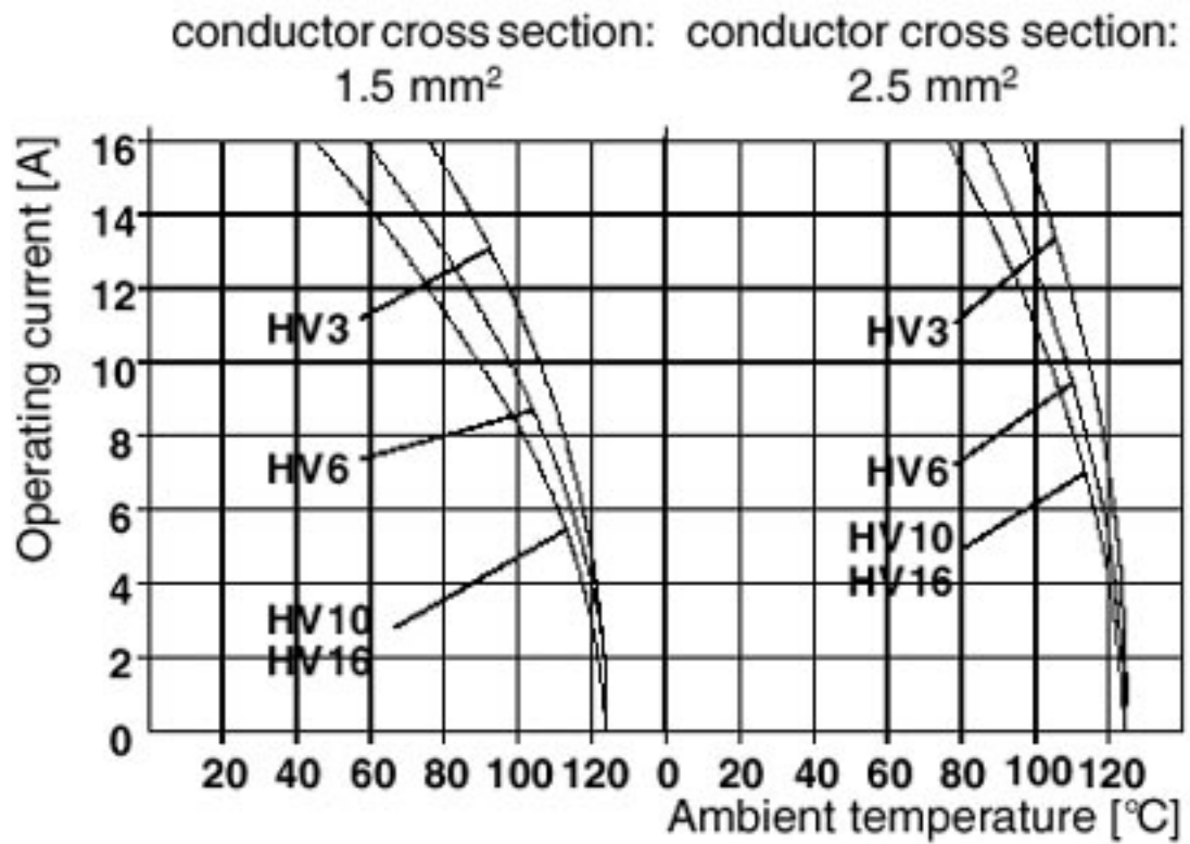
Derating diagram
