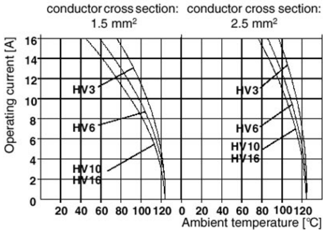
Derating diagram
