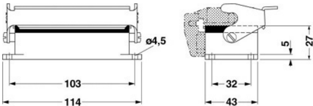
Dimensioned drawing
