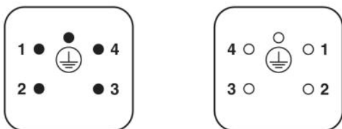
Connector pin assignment connection side: Left pin; right socket
