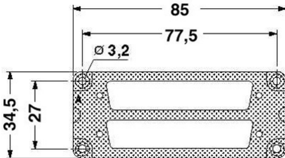
Dimensioned drawing
