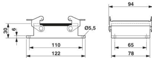
Dimensional drawing
