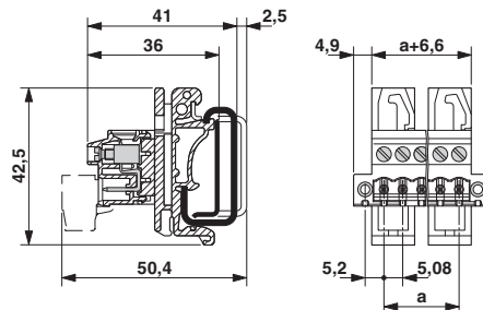
Dimensioned drawing
