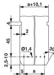
Drilling diagram
