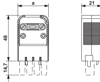
Dimensional drawing
