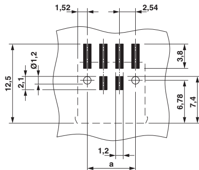
Drilling diagram
