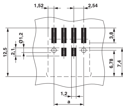
Drilling diagram
