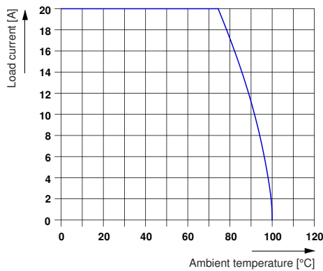
Derating curve VC-TFS 2 / VC-AML 2 / VC-AMS 2
