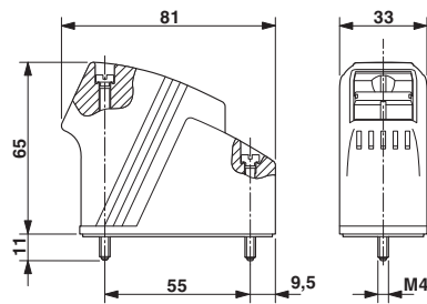
Dimensional drawing
