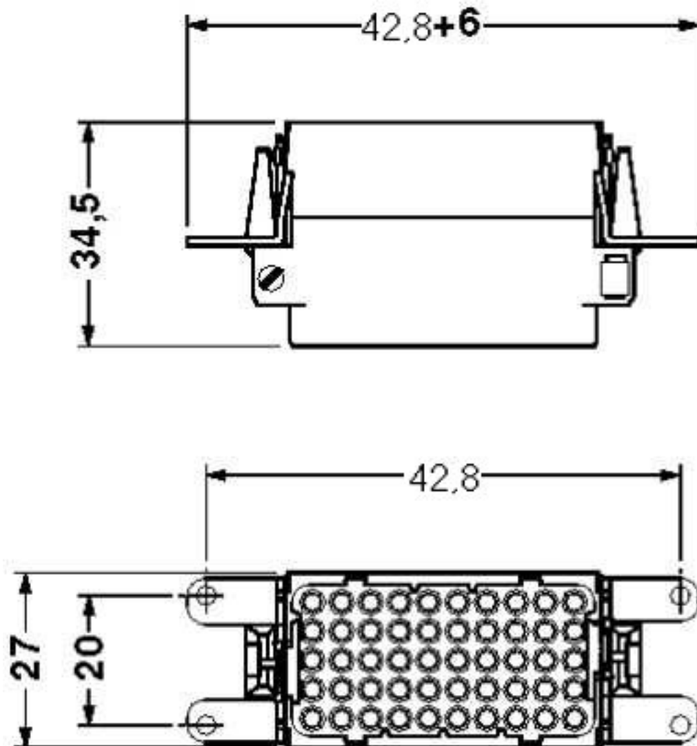
Dimensioned drawing
