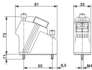
Dimensional drawing
